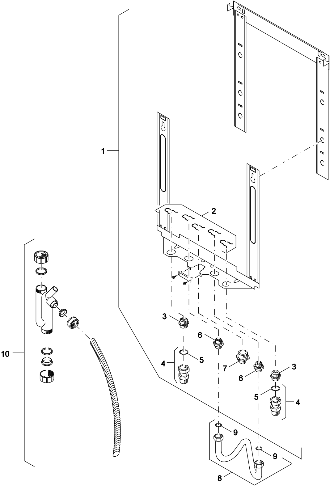
6720906456.aa.RS-Montagerahmen Linea Single
