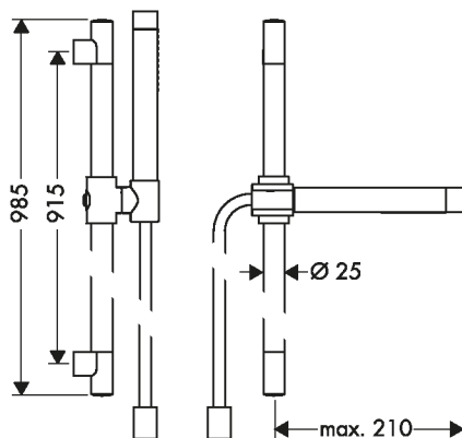
AXOR Starck 27980XX0
