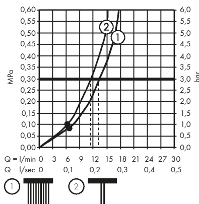
AXOR Starck Organic 12231XX0 (12680XX0)
