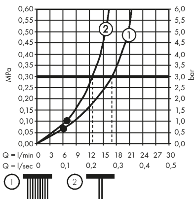
AXOR Starck 27983XX0 (10531XX0)
