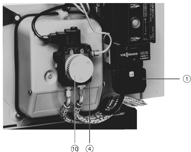
Abb. 12 Ölpumpenfilter
