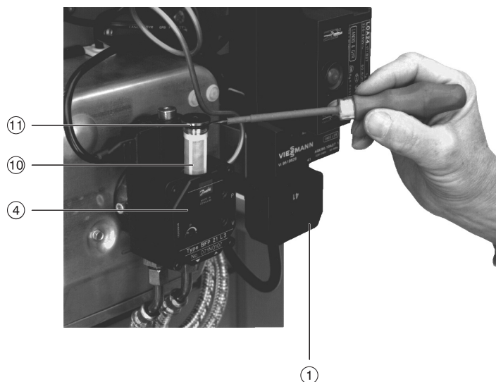
Abb. 11 Ölpumpenfilter
